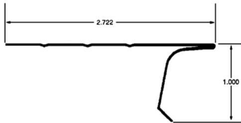
RF130402..120 Overhanging Drip Edge Available in Mill (AE), White (WH), Brown (BN) and Black (BK)
