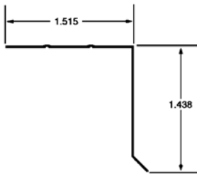
RF130502..120 Improved Roofers Angle Available in Mill (AE), White (WH) and Brown (BN)
