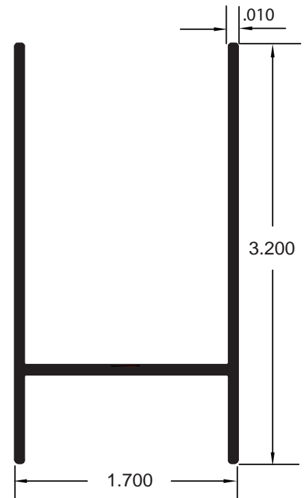
AA020972 H Stiffener 24' Length / AE Finish w/ft. .714
