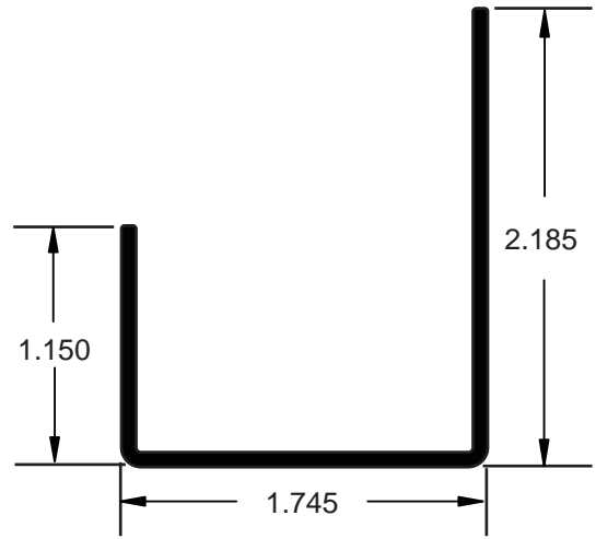
AA020531 J Channel Support 24' Length / AE Finish w/ft. .410
