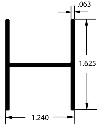
AA018793 H Stiffener 24' Length / AE Finish w/ft. .329
