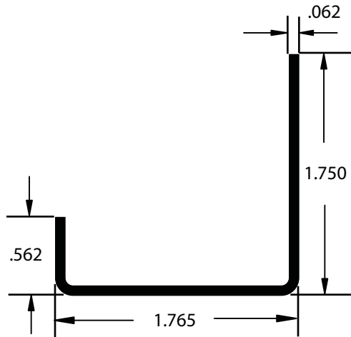
AA018149 J Channel Support 24' Length / AE Finish w/ft. .433
