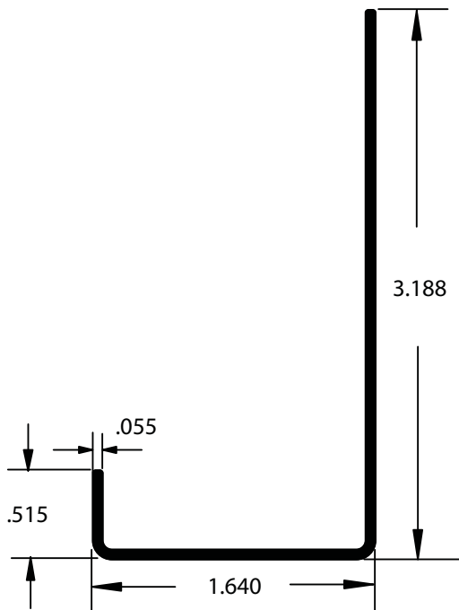
AA019112 J Channel Support 24' Length / AE Finish w/ft. .341
