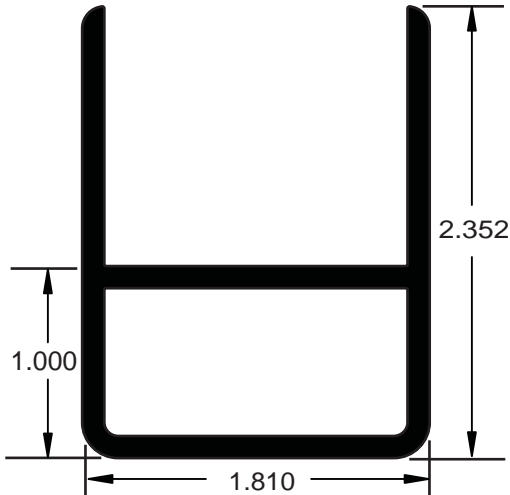
AA020753 U Channel Support 24' Length / AE Finish w/ft. 1.063
