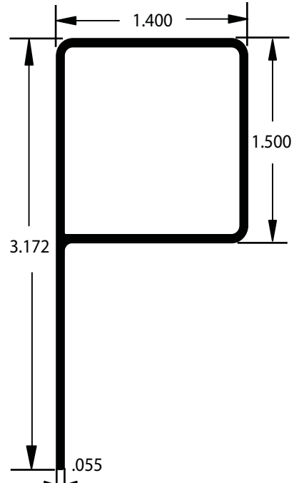
AA019859 P Stiffener 24' Length / AE Finish w/ft. .472
