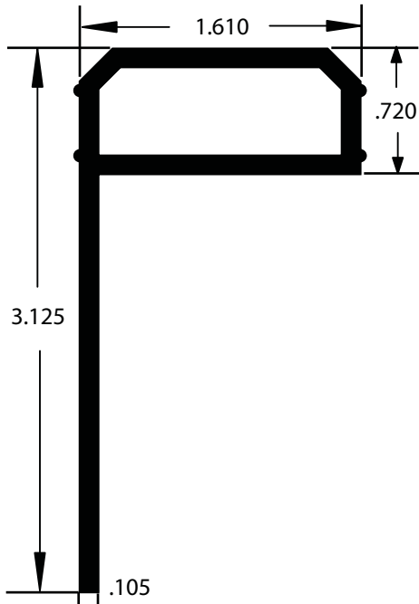
AA019056 P Stiffener 24' Length / AE Finish w/ft. .821
