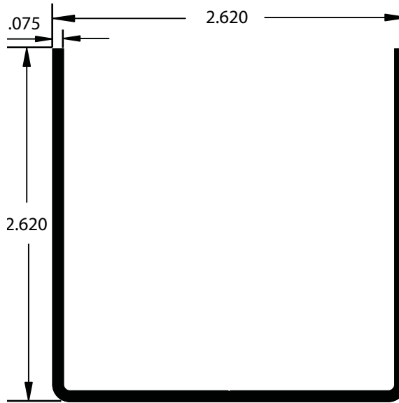
AA018148 U Channel Support 24' Length / AE Finish w/ft. .688
