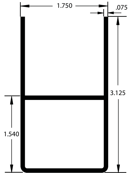
AA018714 U Channel Support 24' Length / AE Finish w/ft. .844
