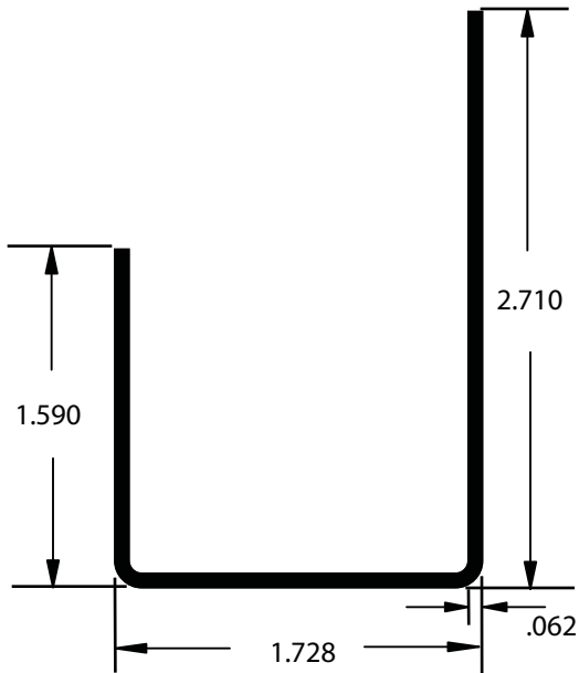
AA018149 J Channel Support 24' Length / AE Finish w/ft. .433
