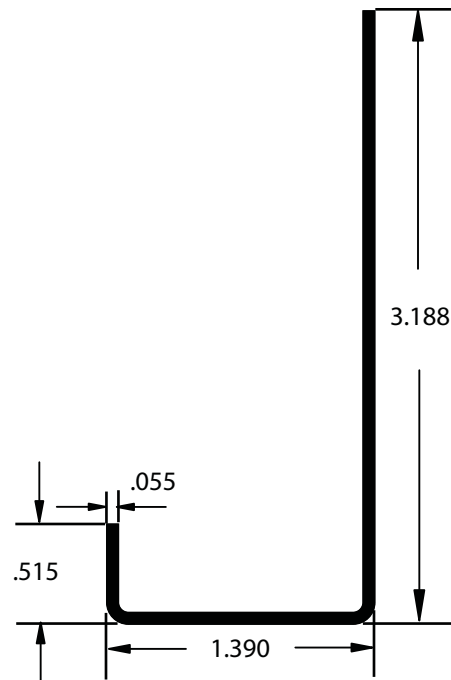
AA018379 J Channel Support 24' Length / AE Finish w/ft. .324
