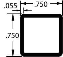
AA018802 Square Tube w/ft. .180
