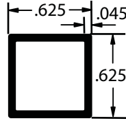
AA018650 Square Tube w/ft. .125
