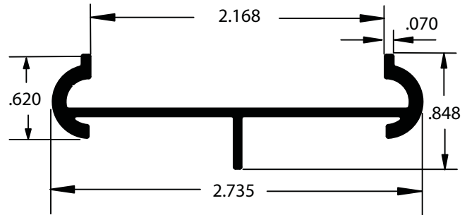
OA002175 Top Rail Support 24' Length / AE Finish w/ft. .397
