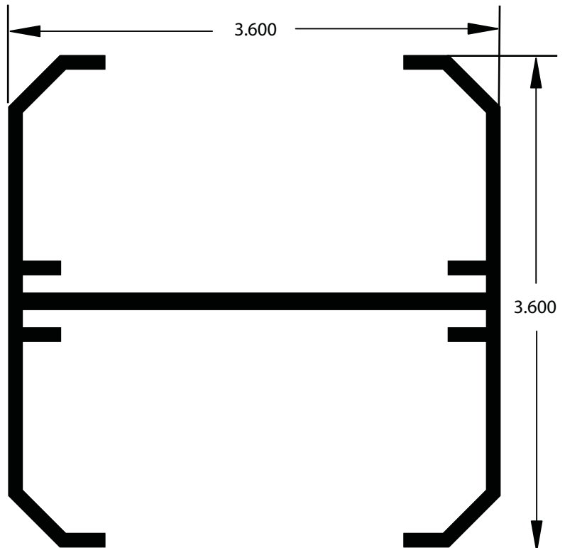
AA019054 4" Post Stiffener 24' Length / AE Finish wall thickness .100 w/ft. 1.591
