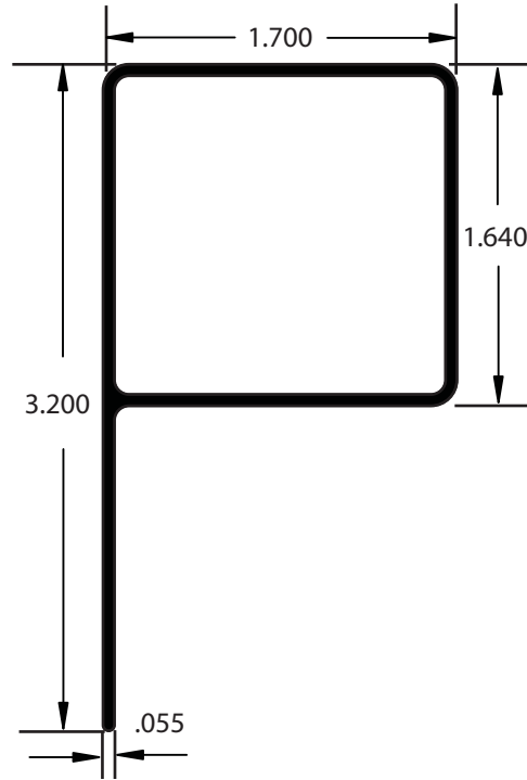
AA020152 P Stiffener 24' Length / AE Finish w/ft. .523
