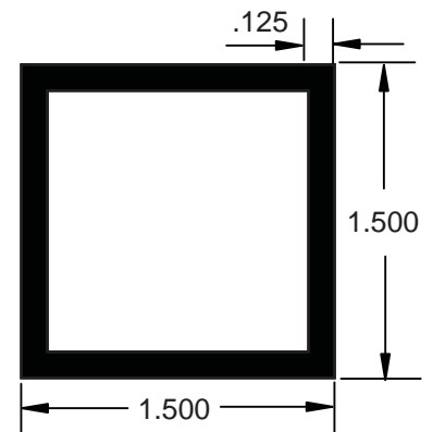
AA008222 Square Tube w/ft. .826
