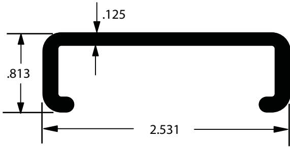
AA019486 Top Rail Stiffener 24' Length / AE Finish w/ft. .646
