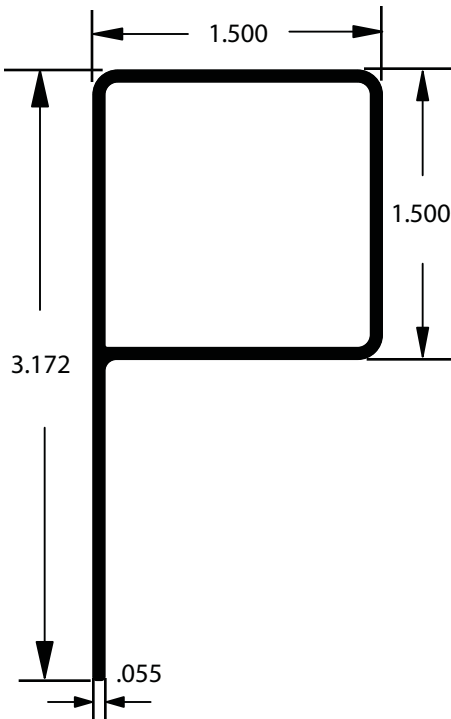
AA019595 P Stiffener 24' Length / AE Finish w/ft. .485
