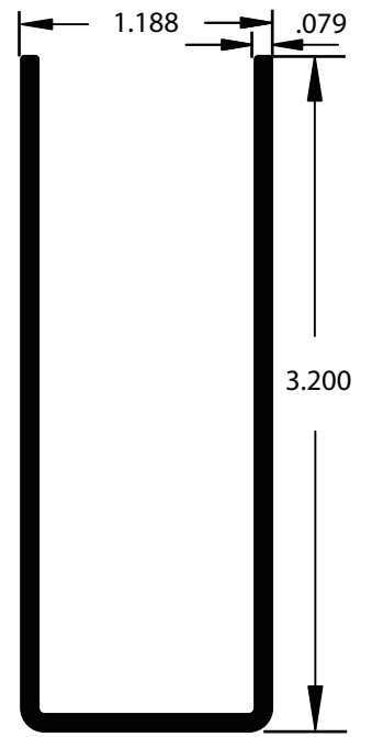
AA018791 U Channel Support 24' Length / AE Finish w/ft. .698
