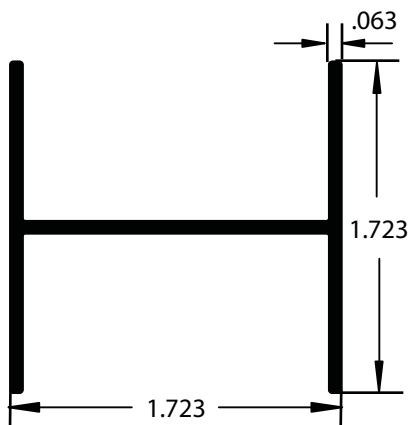
AA018792 H Stiffener 24' Length / AE Finish w/ft. .378
