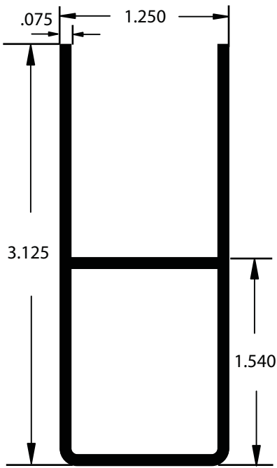
AA018150 U Channel Support 24' Length / AE Finish w/ft. .754
