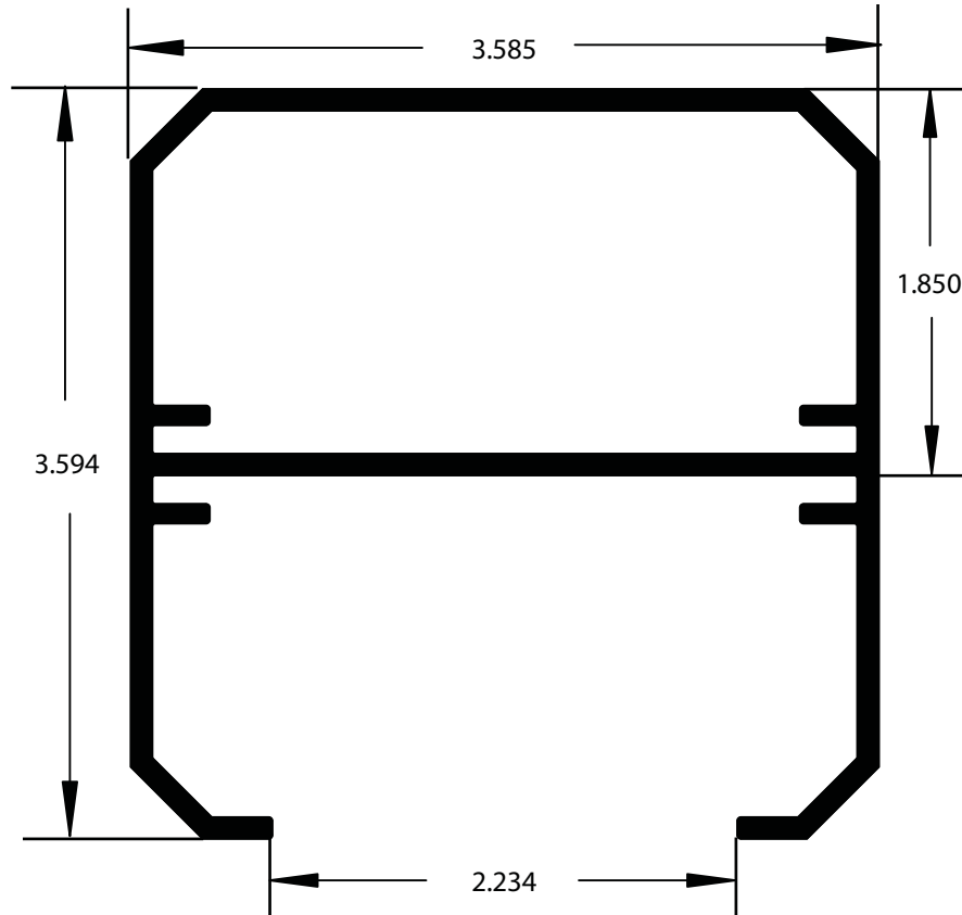
AA019260 4" Post Stiffener with Closed End 24' Length / AE Finish wall thickness .100 w/ft. 1.843
