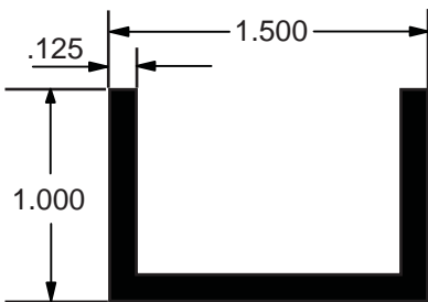
AA008121 U Channel Support 24' Length / AE Finish w/ft. .487
