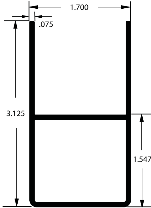
AA019695 U Channel Support 24' Length / AE Finish w/ft. .835
