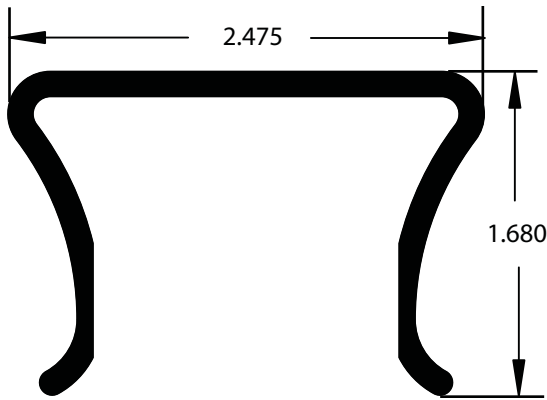
AA018151 Sculptured Channel 24' Length / AE Finish w/ft. .814
