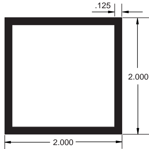
AA008123 Square Tube w/ft. 1.126
