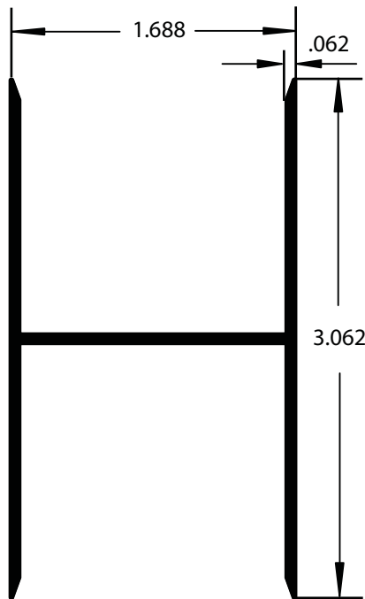
AA018419 H Stiffener 24' Length / AE Finish w/ft. .558
