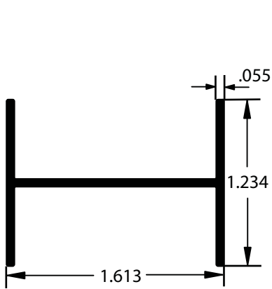
AA019452 H Stiffener 24' Length / AE Finish w/ft. .262
