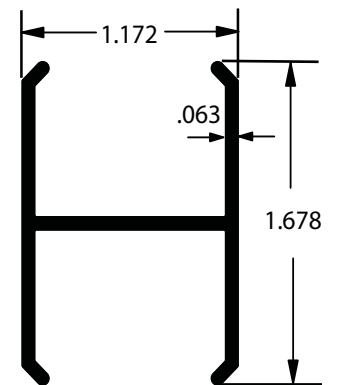
AA019596 HOA Stiffener 24' Length / AE Finish w/ft. .341
