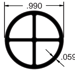
AA020688 Quad Pole used for pool barrier fencing w/ft. .302
