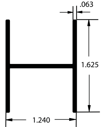
AA018793 H Stiffener 24' Length / AE Finish w/ft. .329
