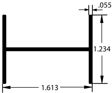
AA019452 H Stiffener 24' Length / AE Finish w/ft. .262
