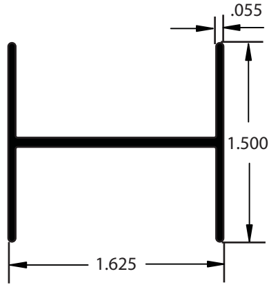
AA020153 H Stiffener 24' Length / AE Finish w/ft. .324
