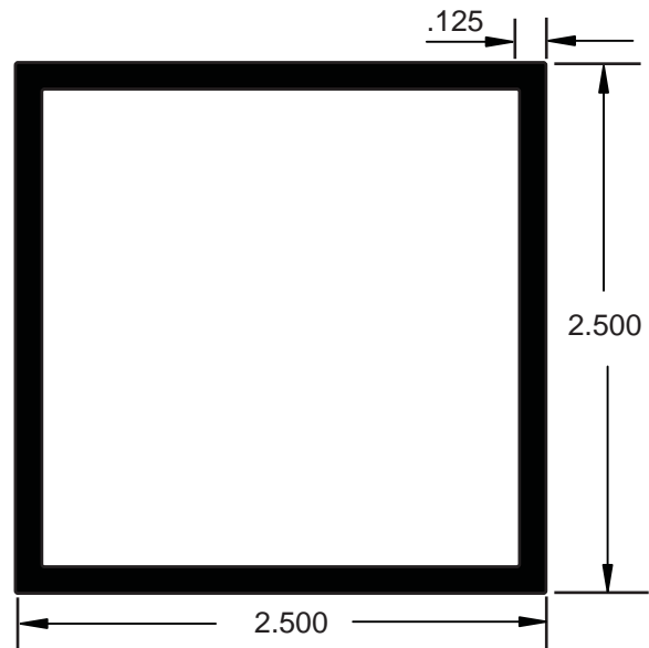
AA019090 Square Tube w/ft. 1.426
