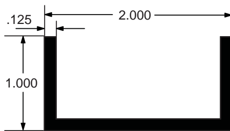
AA000164 U Channel Support 24' Length / AE Finish w/ft. .563
