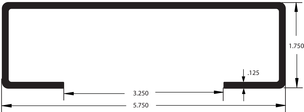
AA020151 Top Rail Stiffener 24' Length / AE Finish w/ft. 1.675
