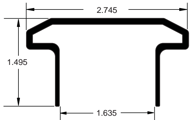
AA020530 Top Rail Stiffener 24' Length / AE Finish w/ft. .654
