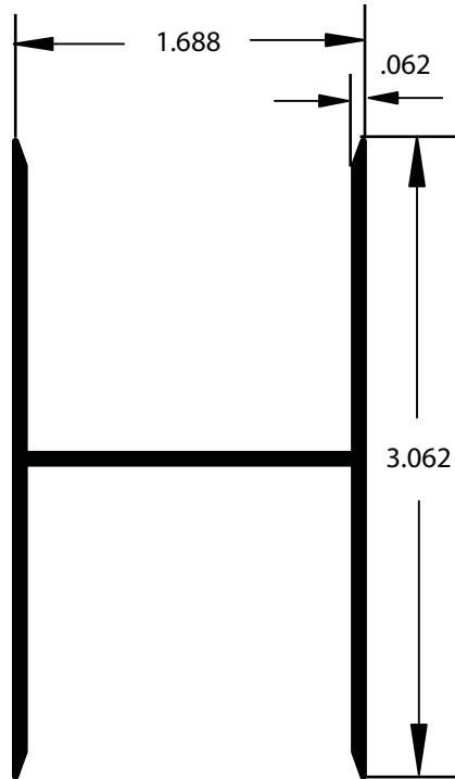
AA018419 H Stiffener 24' Length / AE Finish w/ft. .558
