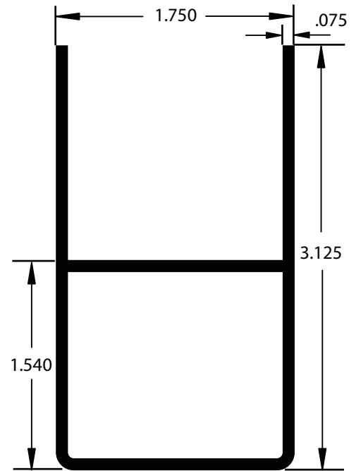
AA018714 U Channel Support 24' Length / AE Finish w/ft. .844
