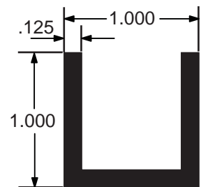
AA000238 U Channel Support 24' Length / AE Finish w/ft. .413
