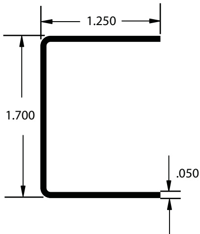
AA019114 Rail Support 24' Length / AE Finish w/ft. .242
