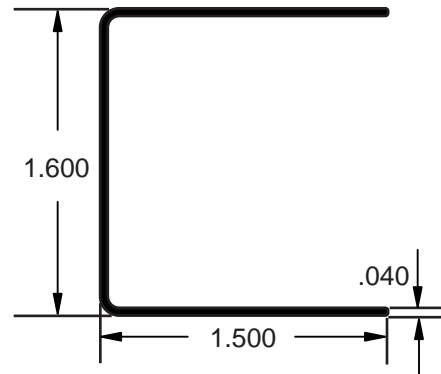
AA020693 Rail Support 24' Length / AE Finish w/ft. .214
