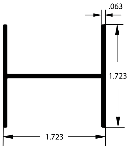
AA018792 H Stiffener 24' Length / AE Finish w/ft. .378
