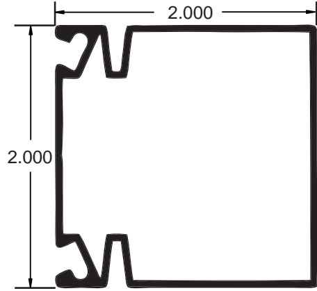
AA021081 2" x 2" Mainframe w/ Kickplate Notch
