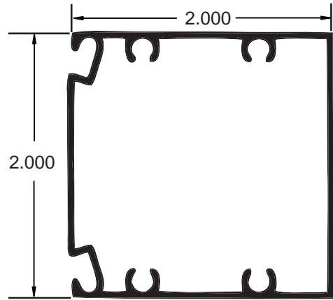
AA021073 2" x 2" Mainframe
