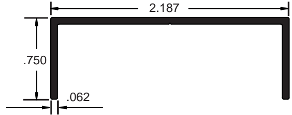
OA099018 2.187" x .75" x .062" U Channel
