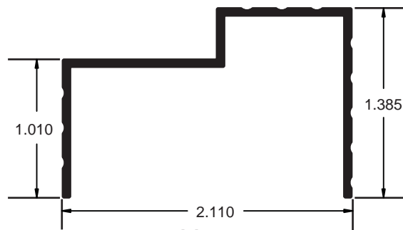
AA020203 Adjustable Z Bar
