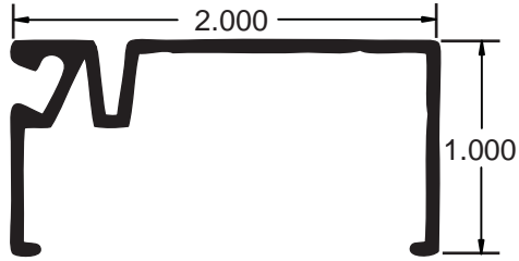
OA099000 1" x 2" Open Back w/ Kickplate Slot
