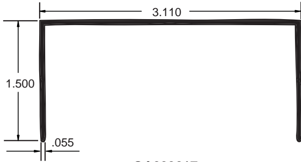
OA099017 3" x 1.5" x .055" Channel
