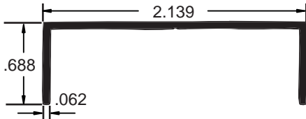
OA099016 2.015" x .688" x .062" Channel
