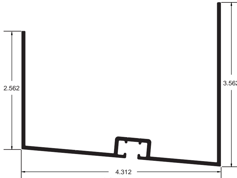
OA099012 4" Wall Mount
