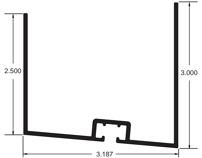
OA099011 3" Wall Mount
