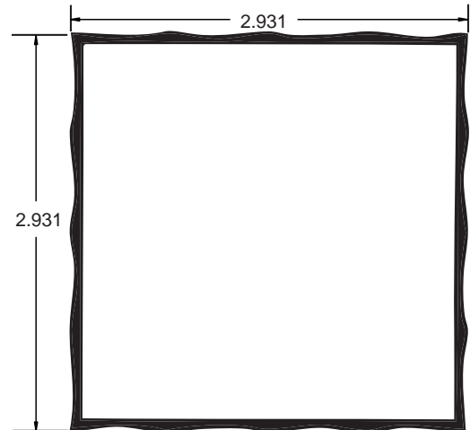
OA099019 3" x 3" x .078" Fluted Post
