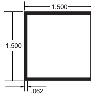
AA011508 1.5" x 1.5" x .062" Tube
