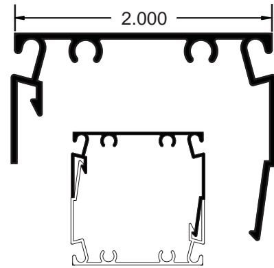
AA019026 2" Snap Post
