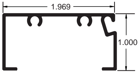
AA019286 1" x 2" Open Back
