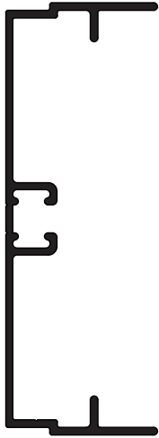
OA045847 3" Male Snap Corner
