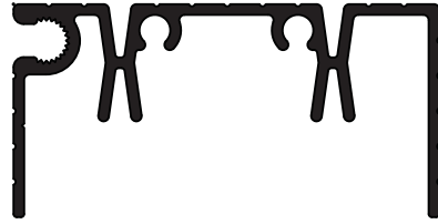
OA045844 2" Female Snap Corner (mates with OA045843)
